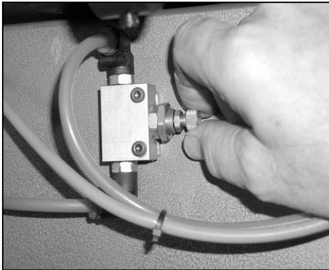
Figure 15. Spindle adjustment.
