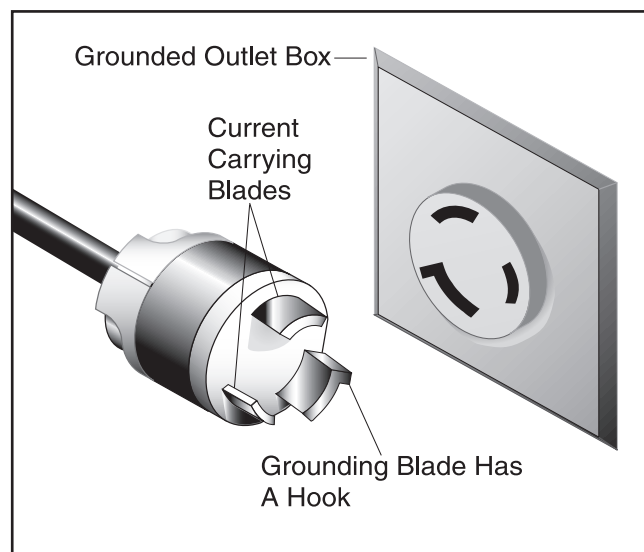
Figure 2. Recommended 220V receptacle.
