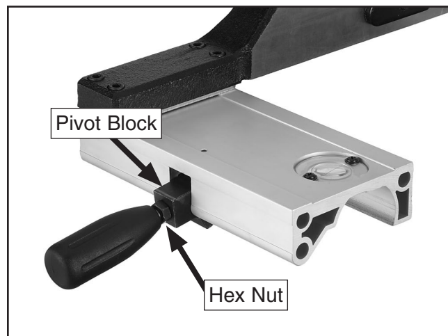
Figure 17. Fence lock lever installed on fence assembly.
