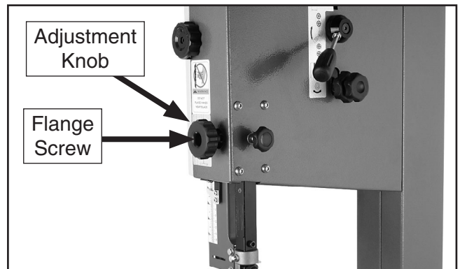
Figure 10. Guide post adjustment knob installed.
