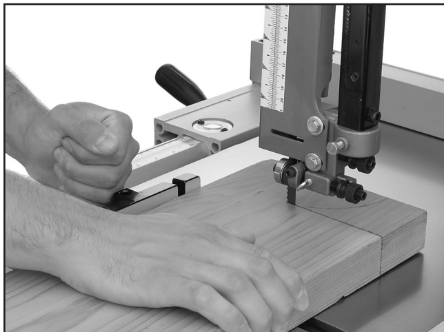
Figure 39. Crosscutting with miter gauge.
