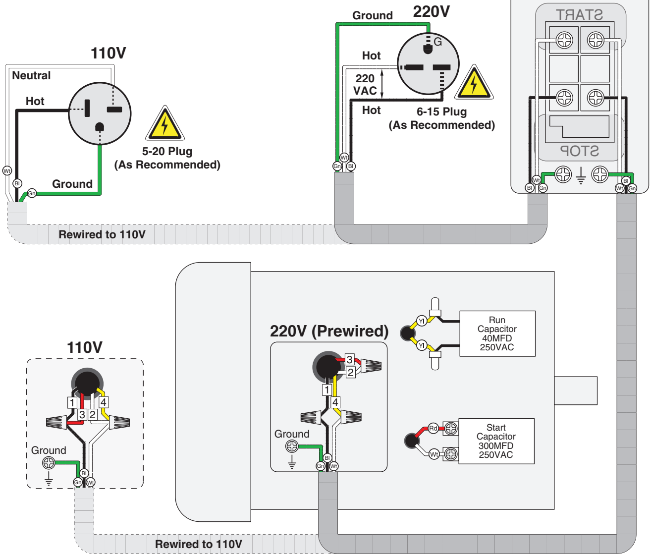
PUSH BUTTON SWITCH (viewed from behind)
