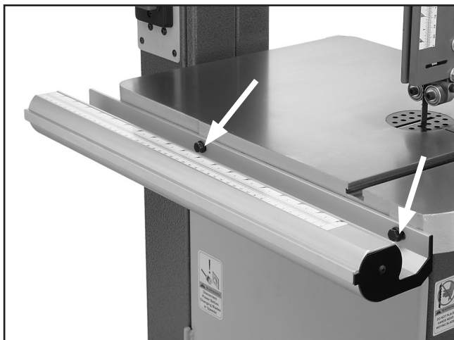
Figure 16. Installed front rail.
