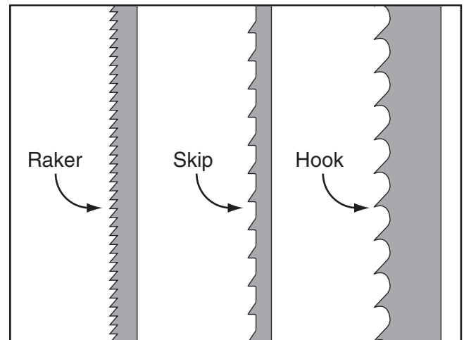
Figure 43. Raker, Skip & Hook tooth styles.
