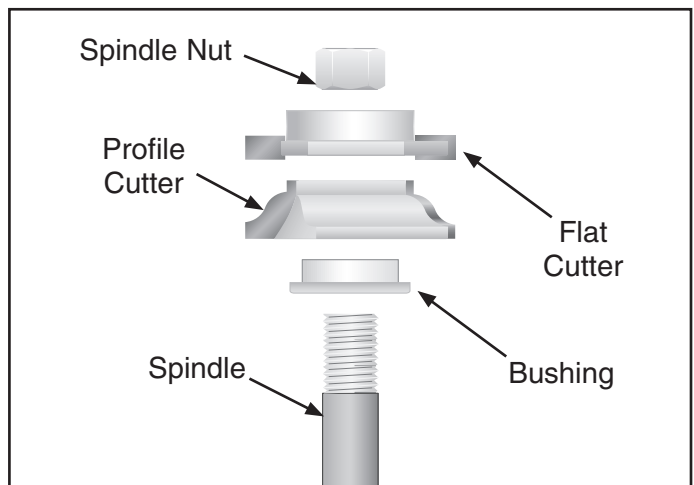
Figure C. Set-up for cutting stiles.
